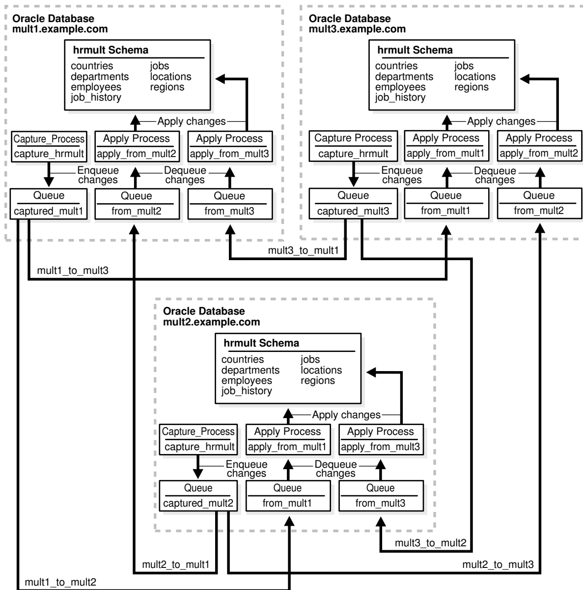
Figure 3-1 Sample N-Way Replication Environment
