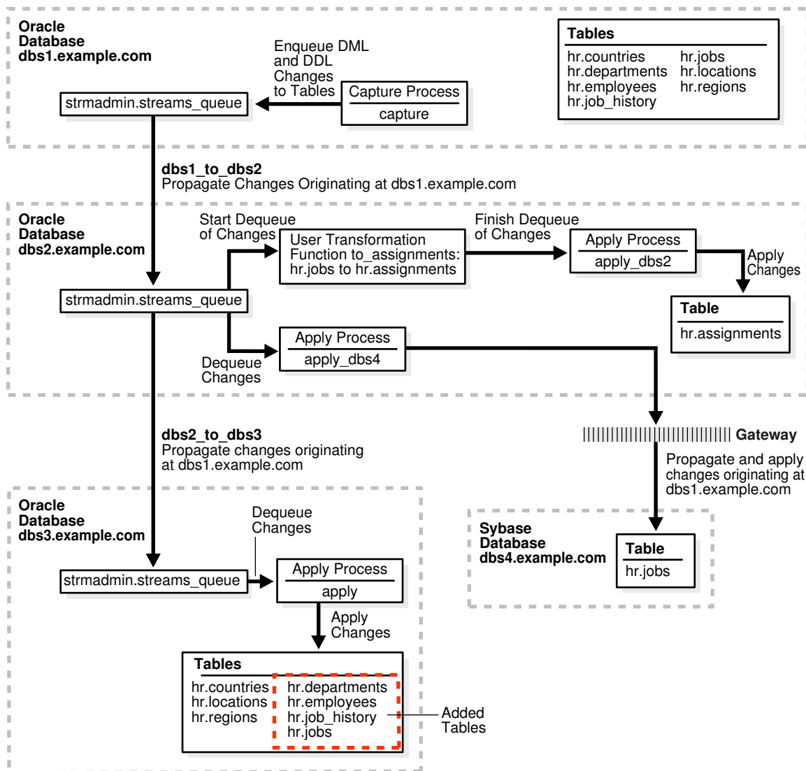
Figure 2-2 Adding Objects to dbs3.example.com in the Environment
